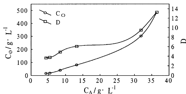
Fig. 6. Extraction of primary crystal from butanol-process by mixed long-chain alcohol.
